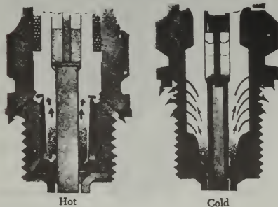
FIGURE 4-26. Hot and cold spark plugs.
